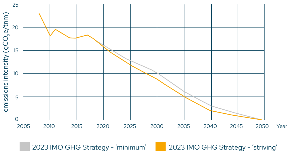
Figure 18. Global fleet’s emission intensity targets and trajectories defined by the 2023 IMO GHG Strategy (grams of well-to-wake CO 2 e per metric tonne-nautical mile [gCO 2 e/tnm])
